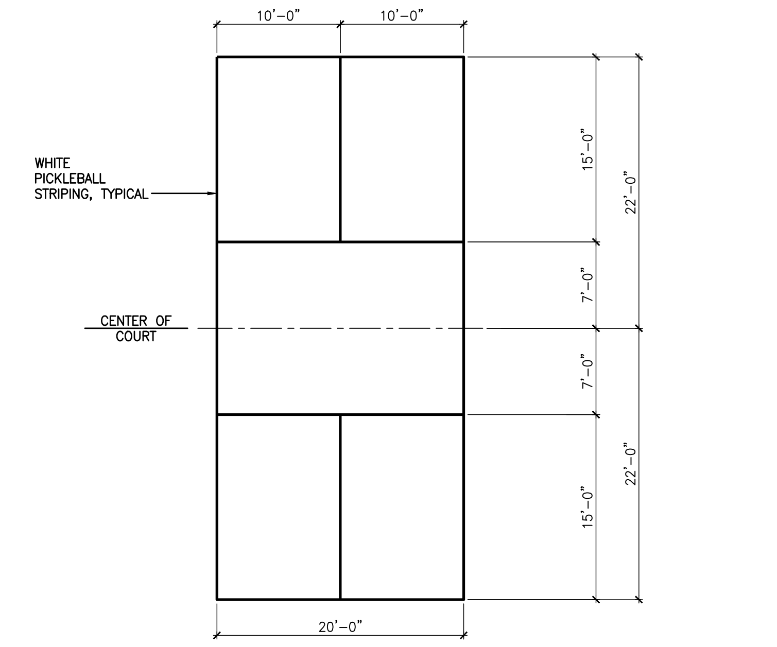
1 PICKLEBALL COURT LAYOUT SCALE: 1/8"=1'-0"
