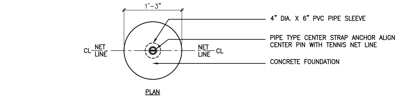
2 NET POST DETAIL SCALE: 1"=1'-0"
