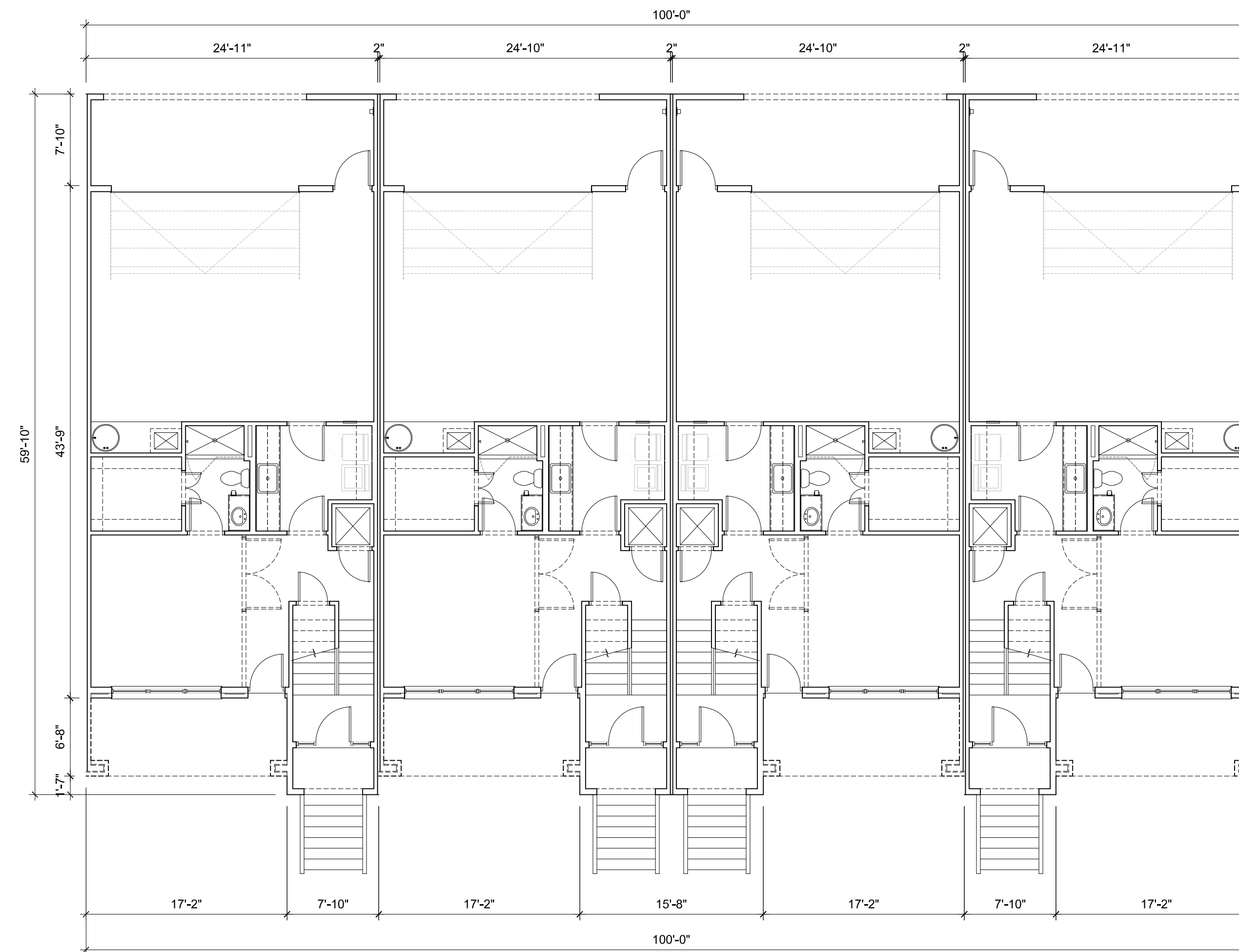
BUILDING TYPE 'D' - GROUND FLOOR SCALE 1/8" = 1'-0"
